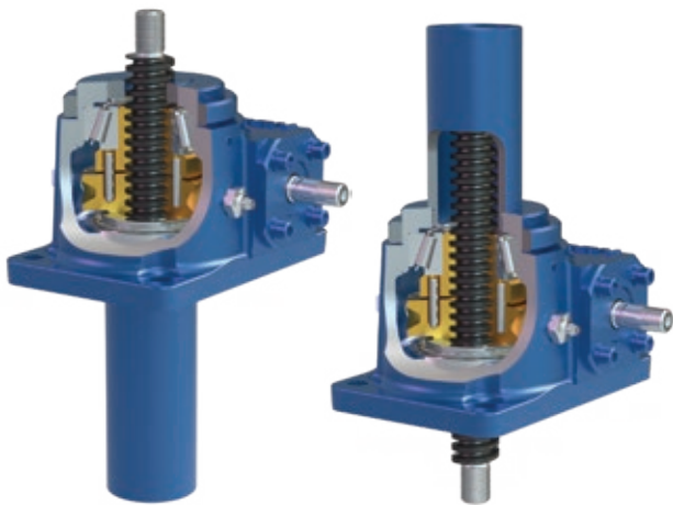
Upright anti-backlash machine screw jack
