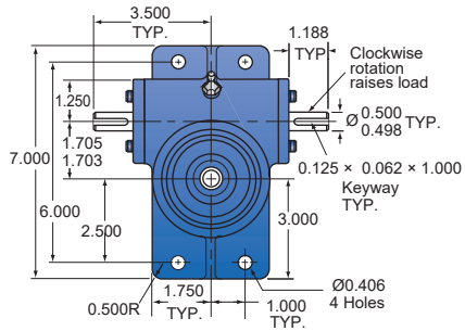
Upright ant-backlash models 2RAB-MSJ-U
