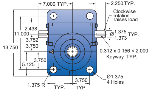
Upright ant-backlash models 30AB-MSJ-U
