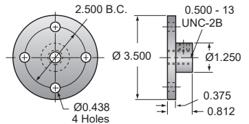
Top plate (optional) 1-BSJ
