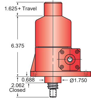
Inverted models 2.5HL-BSJ-I
