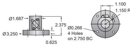
Ball nut and flange 2R-BSJ
