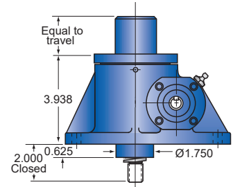
Inverted models 2R-MSJ-I
