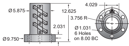
Ball nut and flange 50-BSJ
