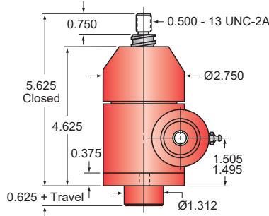
Upright models 1-BSJ-U
