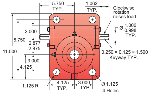
Top view 20-BSJ / 20HL-BSJ
