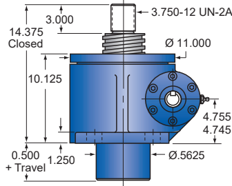
Upright models 50-MSJ-U
