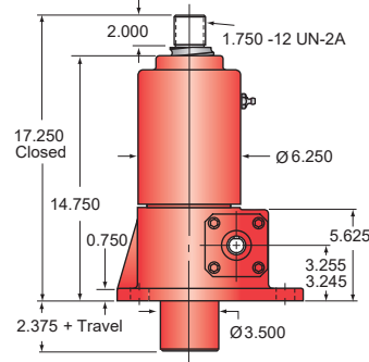
Upright models 20-BSJ-U / 20HL-BSJ-U
