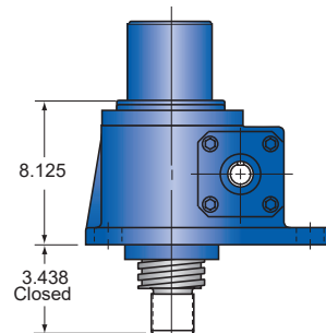
Inverted ant-backlash models 30AB-MSJ-I
