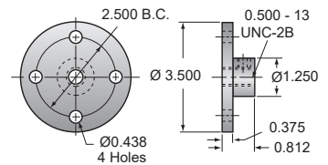
Top plate (optional) 1HL-BSJ
