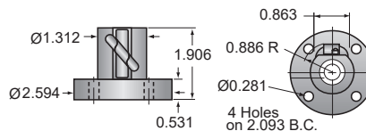
Ball nut and flange 1HL-BSJ
