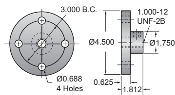
Top plate (optional) 5SS-MSJ
