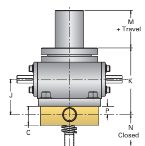
MSJ-I (Machine Screw Inverted)
