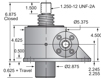
Upright models 10SS-MSJ-U
